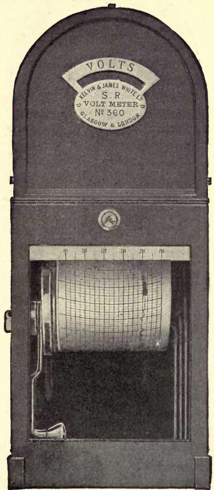
Fig. 200.—Kelvin Permanent-Magnet Moving-Coil Recording Voltmeter
